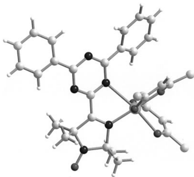
Figure 1. Crystal structure of the copper complex 4 of 4-(4,6-diphenyl-1,3,5-triazin-2-yl)-2,2,5,5-tetramethyl-2,5-dihydroimidazol-1-oxyl ( 3a ) and hfac
