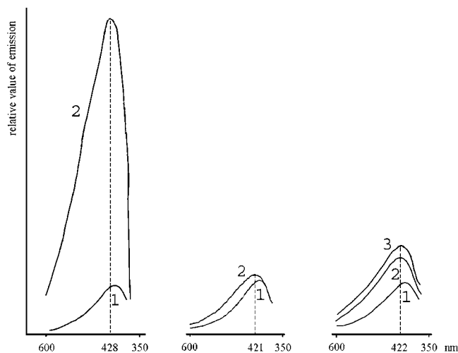
Figure 3. Fluorescence spectra (methanol, 10^{-4} M): 1 – background; left: 2 – methoxy-substituted triazine 3d ; center: 2 – triazine 3a ; right: 2 – oxazole 2a , 3 – oxazole 2a after addition of hydrazine hydrate (3 equiv.)
