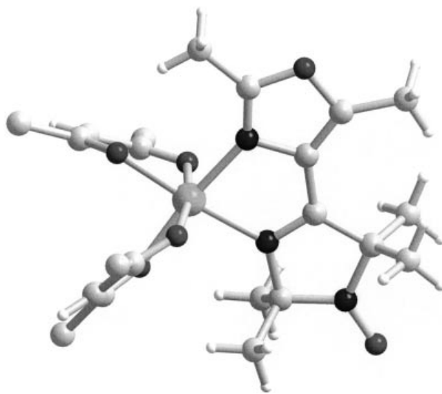
Figure 2. Crystal structure of the copper complex 6 of 4-(2,5-dimethyloxazol-4-yl)-2,5,5-trimethyl-2,5-dihydroimidazol-1-oxyl ( 2b ) and hfac (fluorine atoms omitted)
